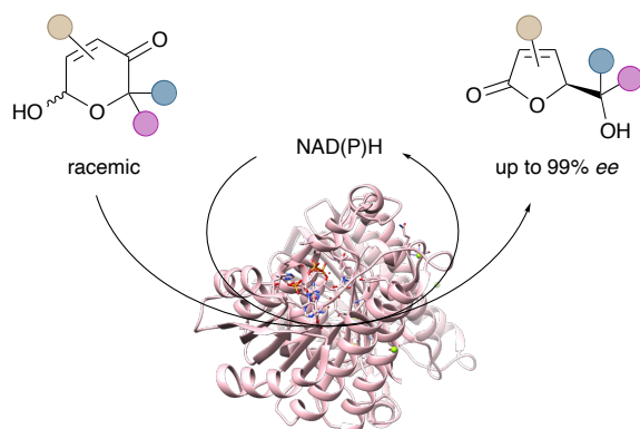
Scheme 1 Redox-neutral enzymatic ring contractions based on the borrowing hydrogen principle: a) in vivo production of rare carbohydrates; b) general biocatalysis tool for the preparation of enantioenriched \gamma -butenolides.
