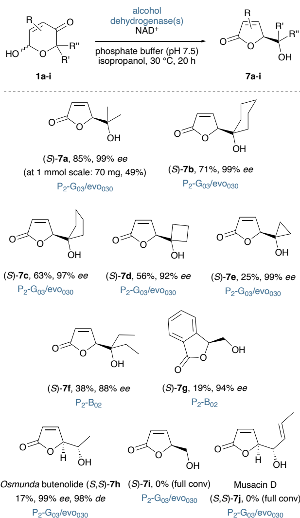
Scheme 4 Scope & limitations of the ADH-mediated ring contraction. Reaction conditions: 1 (10–20 mg) P_2\text{-G}_{03}/\text{evo}_{030} (1.5 mg/mL each) or P_2\text{-B}_{02} (1.5 mg/mL), \text{NAD}^+ (0.6 mg/mL), i\text{PrOH} 20 \mu\text{L/mL} \text{KPi} buffer (1 ml/mg 1 , 50 mM, pH 7.5), 30 ^{\circ}\text{C} , 20 h; isolated yields after column chromatography. Absolute configurations were assigned in analogy to the non-contracted \delta -lactones 2 which were produced by the same set of dehydrogenases and of which the stereochemistry was studied by vibrational circular dichroism; 47 all products that were not part of the VCD study were assigned based on HPLC elution order.
