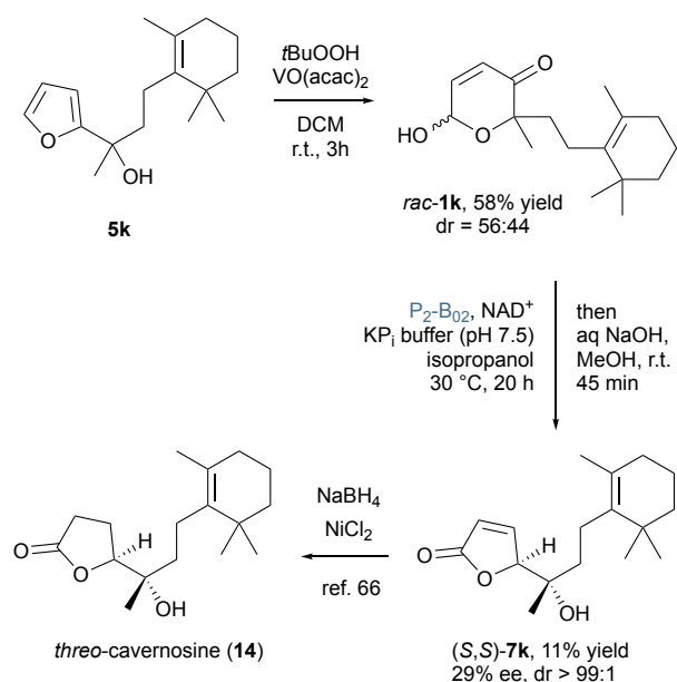
Scheme 6 Chemoenzymatic formal total synthesis of threo -cavernosine
