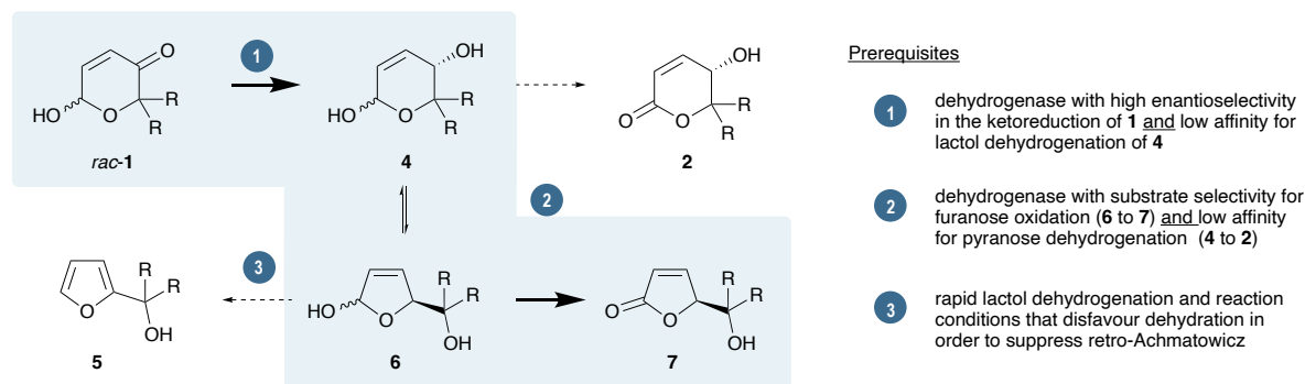
Scheme 2 Development of a blueprint for the investigation of an enantioselective butenolide synthesis through borrowing hydrogen ring contraction
