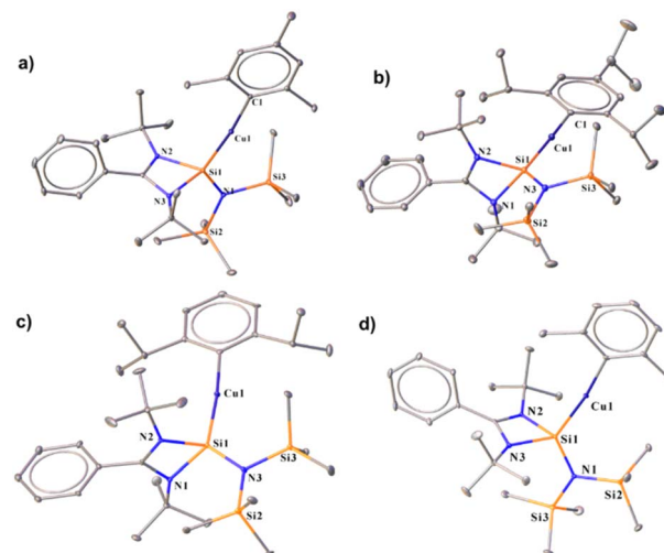
Fig. 1 Molecular structures of 2 (a), 3 (b), 4 (c), and 5 (d). The bond distance (Å) and bond angle ( ^\circ ) are discussed in the ESI.†
