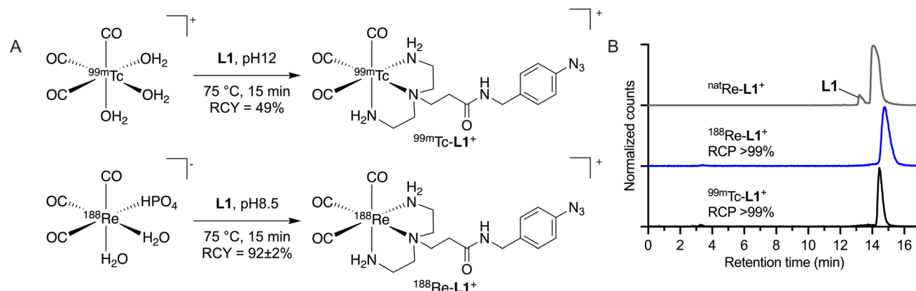
Fig. 4 Radiosynthesis of the \text{M-L1}^+ complexes ( \text{M} = {}^{99\text{m}}\text{Tc} , {}^{188}/{}^{186}\text{Re} ) showing (A) the synthetic procedures employed and (B) (radio-)HPLC chromatograms of {}^{99\text{m}}\text{Tc-L1}^+ , {}^{188}\text{Re-L1}^+ , and {}^{\text{nat}}\text{Re-L1}^+ (UV trace, 254 nm).
