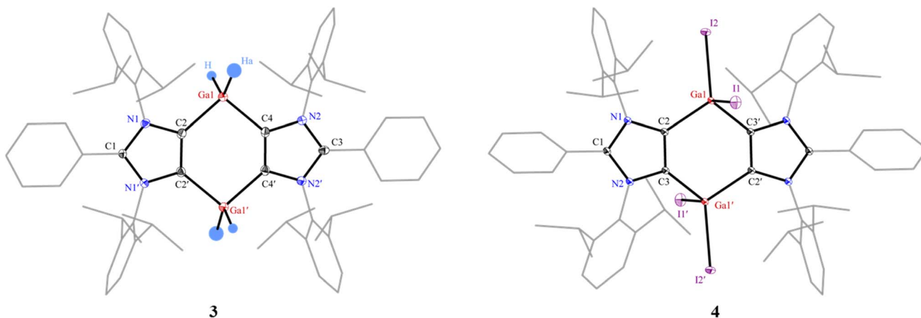
Fig. 2 Solid-state molecular structures of 3 and 4 . Hydrogen atoms (except on GaH 2 for 3 ) and two benzene molecules (for 3 ) are omitted for clarity. Aryl groups are depicted as wireframes. Thermal displacement ellipsoids at 50%. Selected bond lengths (Å) and angles (°) for 3 : C2–Ga1 2.016(3), C4–Ga1 2.015(3), C2'–C2 1.377(6), C2–Ga1–C4 101.2(1), symmetry code: 2 - x, 1 - y, z ; and for 4 : C2–Ga1 1.993(1), C3'–Ga1 1.993(1), Ga1–I1 2.6117(1), Ga1–I2 2.5230(1), C2–C3 1.378(1), I1–Ga1–I2 107.47(1), C2–Ga1–I1 100.14(2), C2–Ga1–I2 117.85(2), C2–Ga1–C3' 107.36(3), symmetry code: 1 - x, 1 - y, 1 - z .
