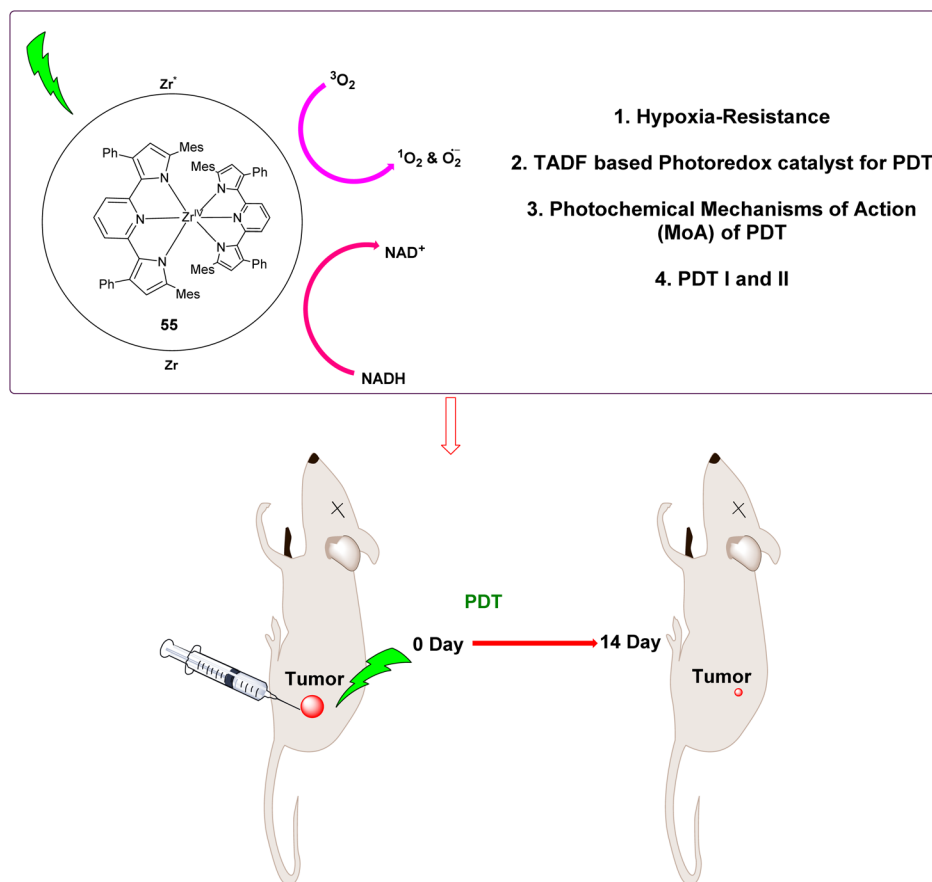
Fig. 39 Schematic representation of the TADF-based photocatalyst Zr(MesPDPPh) 2 NPs and its use in PDT. Reproduced from ref. 204 with permission from American Chemical Society, Copyright © 2023.
