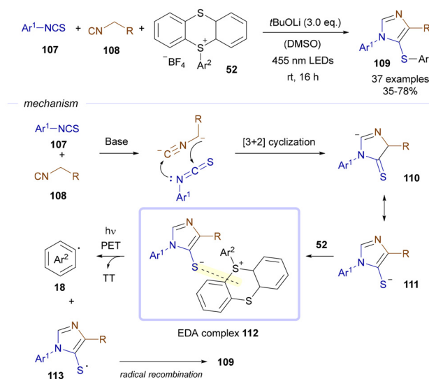
Scheme 16 One-pot multicomponent reaction of isothiocyanates 107 , isocyanides 108 , and thianthrenium salts 52 to prepare trisubstituted imidazoles 109 .
