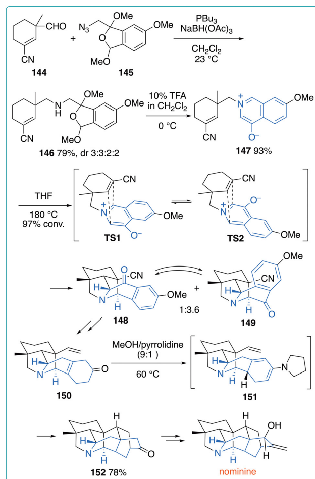
Fig. 21 Gin's total synthesis of nominine.
