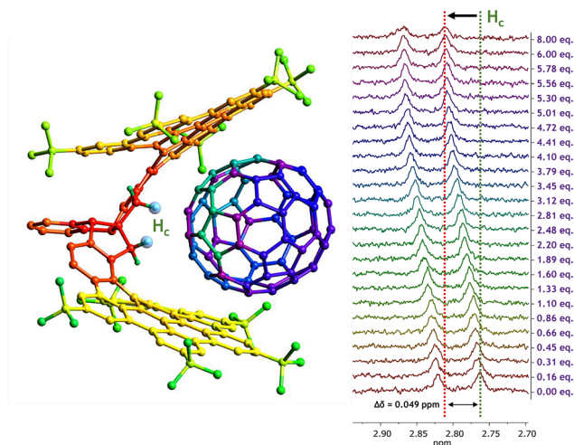
Fig. 3 Model for the supramolecular complexation of the CNG-1 ⊃ C 70 complex with a 1:1 stoichiometry (left), and 1 H c signal chemical shift variation upon addition of C 70 equivalents throughout the titration in PhCl- d 5 (right).
