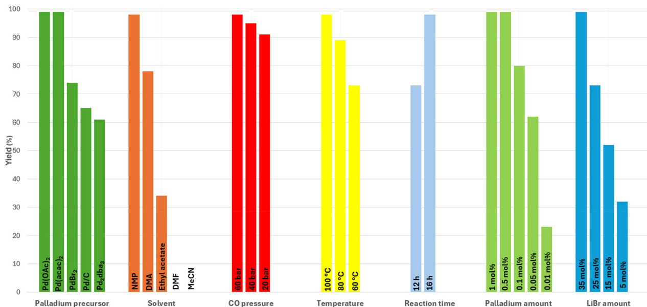
Fig. 3 Palladium-catalyzed amidocarbonylation of dodecanal with acetamide: variation of reaction conditions. Reactions were conducted on a 0.5 mmol scale and yields were determined by ^1\text{H} -NMR analysis using 3,5-bis(trifluoromethyl)bromobenzene as an internal standard.
