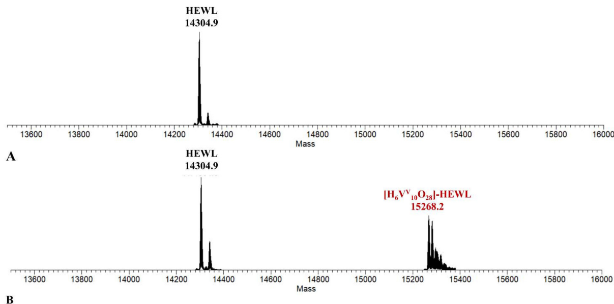
Fig. 5 Deconvoluted ESI-MS spectra of HEWL (concentration = 13 mg mL -1 ) (A) and of the system containing Cs 2 [V 10 O 28 ](mal) 2 ·2H 2 O : HEWL in 1 : 1 molar ratio (B). Both samples were diluted 1 : 100 in acetonitrile/H 2 O + 1% FA. Mass is in Da.
