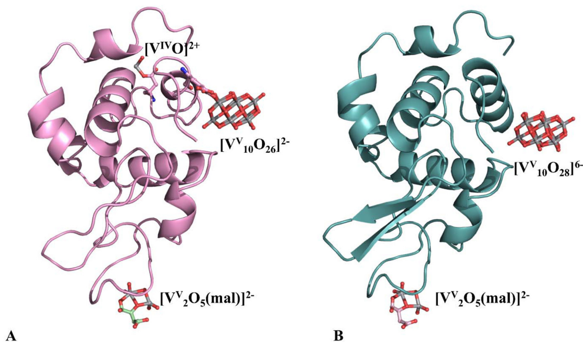
Fig. 6 Overall structures of V-HEWL adducts derived from two crystals of HEWL exposed to Cs 2 [V 10 O 28 ](mal) 2 ·2H 2 O for 7 days: (A) Structure A; (B) structure B. Vanadium atoms are in grey. Coordinates and structure factors were deposited in the PDB under the accession codes 9RBG, and 9RBT.
