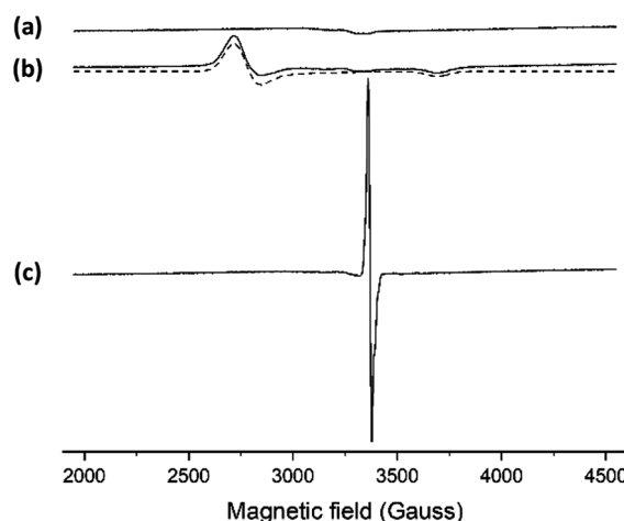
Fig. 4 X-band cw-EPR spectra recorded at 100 K of a MeCN solution of fac -C2 (0.2 mM) containing 0.1 M TBAPF 6 . (a) Initial Fe(II) complex, (b) after exhaustive electrolysis at E_{app} = 1.2 V vs. SCE. Simulation in dashed line for a low-spin S = 1/2 Fe(III) complex with g_{\perp} = 2.452 and g_{\parallel} = 1.823 , (c) after exhaustive electrolysis at E_{app} = -1 V vs. SCE to generate an Fe(II)L •− radical with g = 1.999 .
