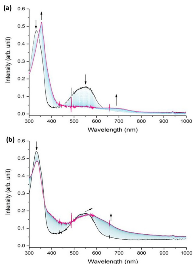
Fig. 3 In situ UV-VIS spectra of fac -C2 (0.2 mM) in an acetonitrile solution containing 0.1 M TBAPF 6 , (a) during exhaustive oxidation at E_{app} = 1.2 V vs. SCE (last scan after 285 s), (b) during exhaustive reduction at E_{app} = -1 V vs. SCE (last scan after 570 s) (pathlength of 1 mm and scan delay of 5 s between two spectra).
