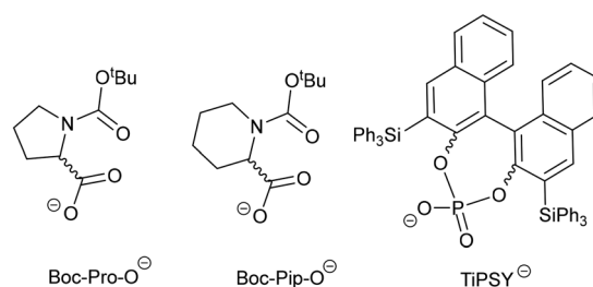
Fig. 4 Chiral anionic ligands for zinc(II). Boc-Pro-O − , Boc-Pip-O − and TIPSYP − are derived from N -(tert-butoxycarbonyl)-proline, N -(tert-butoxycarbonyl)-pipercolic acid and 3,3'-bis(triphenylsilyl)-1,1'-binaphthyl-2,2'-diyl hydrogenphosphate respectively.
