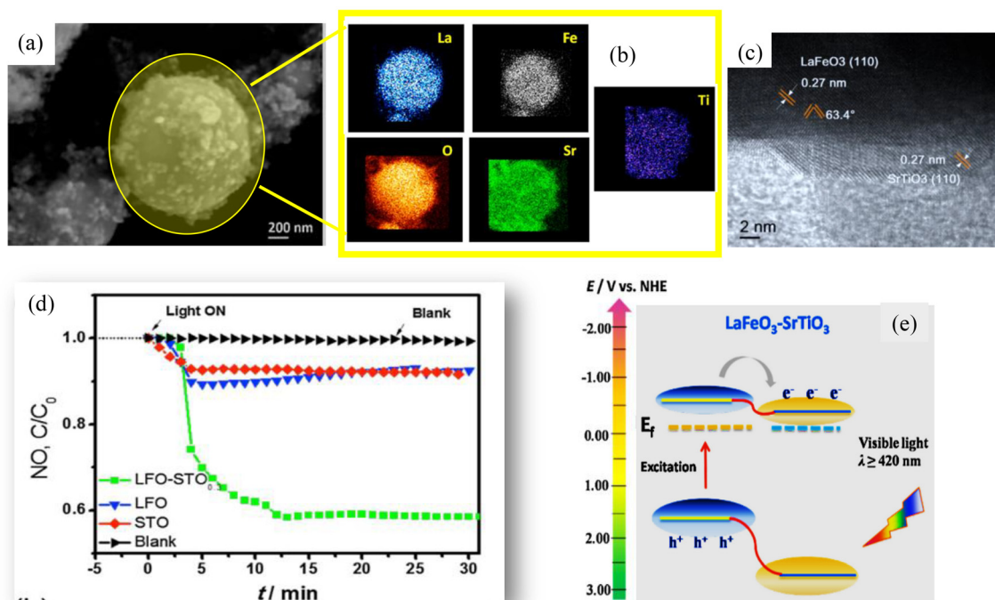
Fig. 5 (a) Representative scanning electron microscopy (SEM) image and (b) the corresponding EDXS chemical maps for a LaFeO 3 -SrTiO 3 heterostructured system, obtained by ultrasonic spray pyrolysis, followed by solvothermal treatment. (c) HR-TEM image of the LFO/STO interface. (d) Photocatalytic NO removal profiles ( C/C_0 ) as a function of time (Vis-light irradiation). (e) Schematic band energy diagram for LFO-STO heterostructures and the corresponding charge carrier separation under Vis illumination. Reprinted with permission from ref. 12. Copyright 2017, Elsevier.
