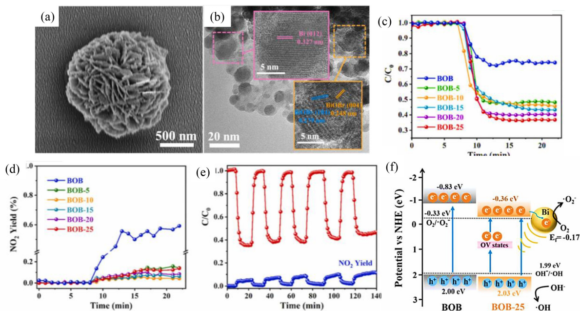
Fig. 7 Characterization of Bi/BiOBr photocatalysts prepared using a solvothermal approach in water–ethanol mixtures [denoted as BOB- x ( x = 0, 5, 10, 15, 20 , and 25 mL of ethanol in an overall solvent volume of 25 mL)]. 18 SEM (a) and TEM (b) images of BOB-25. TEM analyses show two different types of lattice fringes with d spacings corresponding to the (104) and (004) planes of BiOBr ( \approx 0.279 nm and 0.248 nm, respectively). The interplanar spacing of 0.327 nm corresponded to the (012) plane of \text{Bi}^0 , confirming the surface presence of the latter. (c) Photocatalytic NO conversion and (d) the corresponding \text{NO}_2 formation over BOB- x specimens under Vis-light irradiation. (e) Cycling experiments over BOB-25. (f) Schematic energy band diagram, reporting approximate energy levels with respect to the normal hydrogen electrode (NHE) scale. Reprinted with permission from ref. 18. Copyright 2023, Elsevier.
