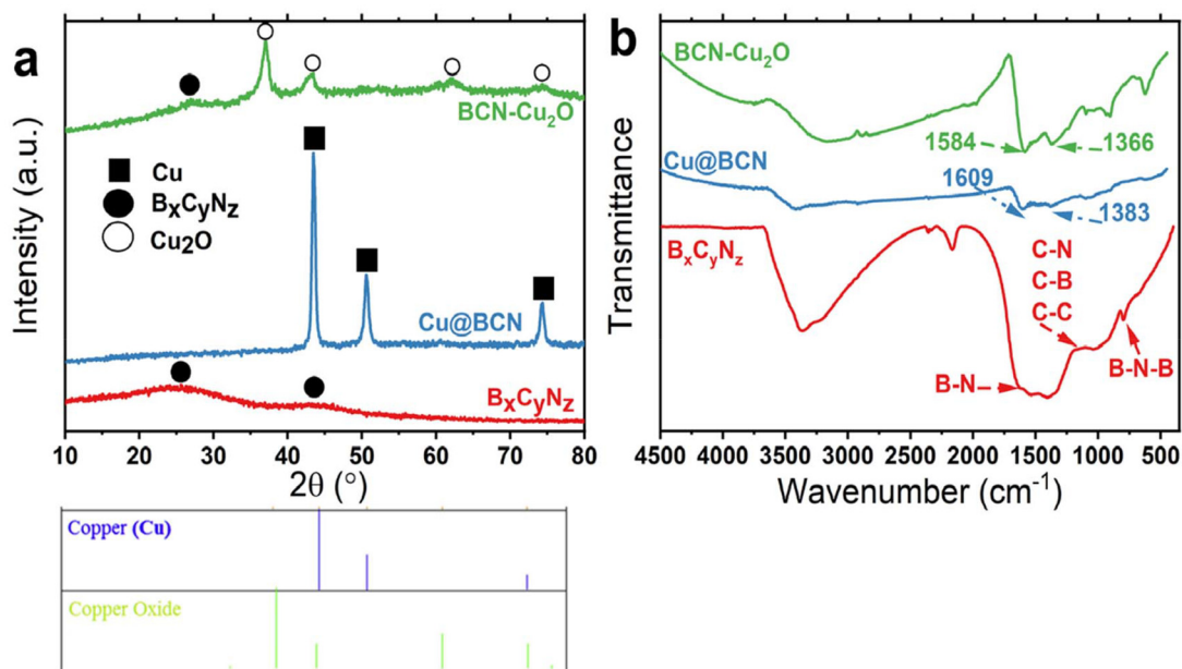
Fig. 5 XRD patterns (a), and FT-IR spectra (b) of the as-prepared BCN500, and the Cu/BCN composites prepared without (BCN-Cu 2 O) and with surface activation (Cu@BCN). XRD patterns of copper and copper oxide are added for comparison.
