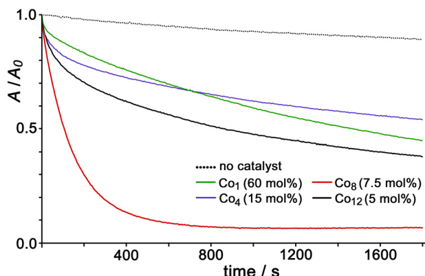
Fig. 7 Normalised UV/vis absorption data showing destruction of FLU ( 7.5 \mu\text{M} , \lambda_{\text{max}} = 489 \text{ nm} ) by oxidation with PMS (45 eq.) over time with no catalyst, Co 12 (5 mol%), Co 8 (7.5 mol%), Co 4 (15 mol%) and Co 1 (60 mol%), with cage concentrations adjusted to give the same concentration of Co(II) centres in each case. Solvent was aqueous buffer containing TWEEN-20 surfactant (see ref. 5a) at pH 7.
