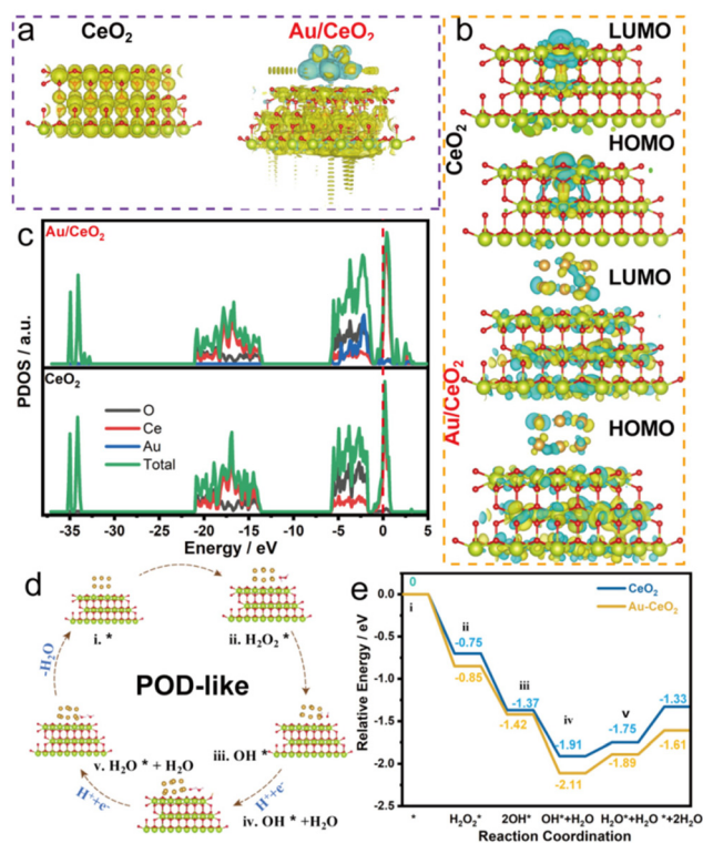
Fig. 5 (a) Charge density difference illustration of \text{CeO}_2 and \text{Au}/\text{CeO}_2 . (b) HOMO–LUMO energy levels and the interfacial diagrams of the molecular orbitals for \text{CeO}_2 and \text{Au}/\text{CeO}_2 . (c) Density of states of \text{CeO}_2 and \text{Au}/\text{CeO}_2 . (d) Proposed reaction pathways of the POD-like reaction. (e) Corresponding free energy diagrams of \text{CeO}_2 and \text{Au}/\text{CeO}_2 for the POD-like reaction.
