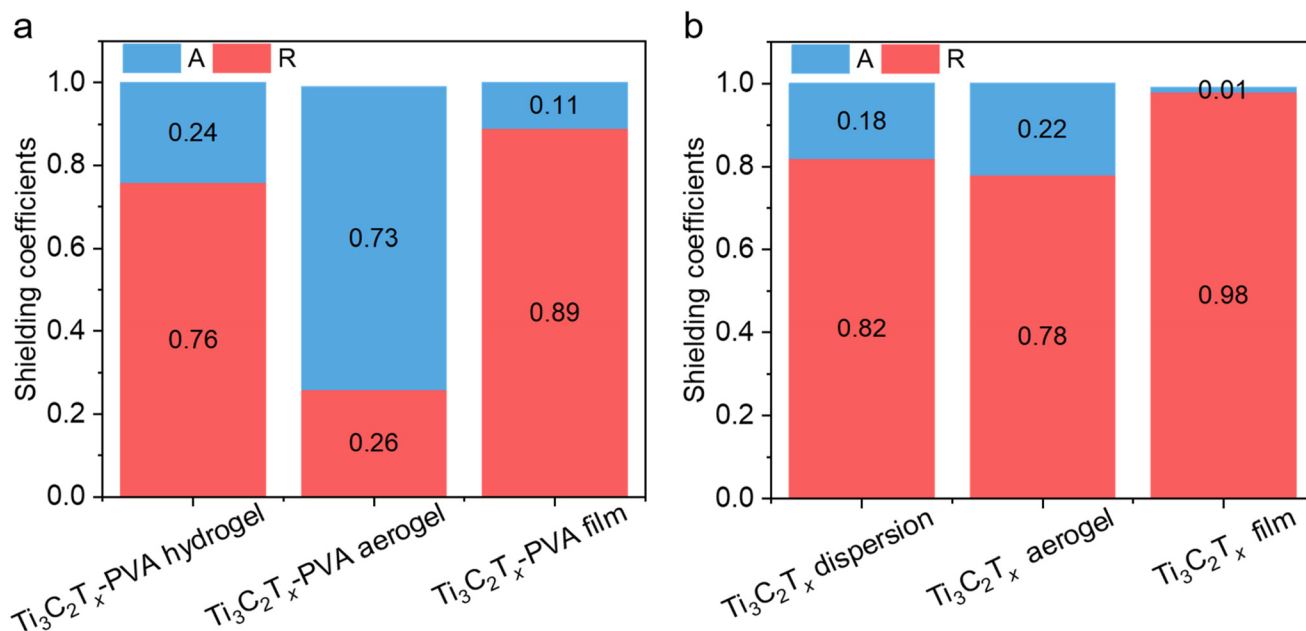
Fig. 5 Absorption coefficient ( A ) and reflection coefficient ( R ) of the (a) \text{Ti}_3\text{C}_2\text{T}_x -PVA-based hydrogel, aerogel, and film and (b) \text{Ti}_3\text{C}_2\text{T}_x -based dispersion, aerogel, and film at a fixed \text{Ti}_3\text{C}_2\text{T}_x areal density ( 20 \text{ mg cm}^{-2} ).
