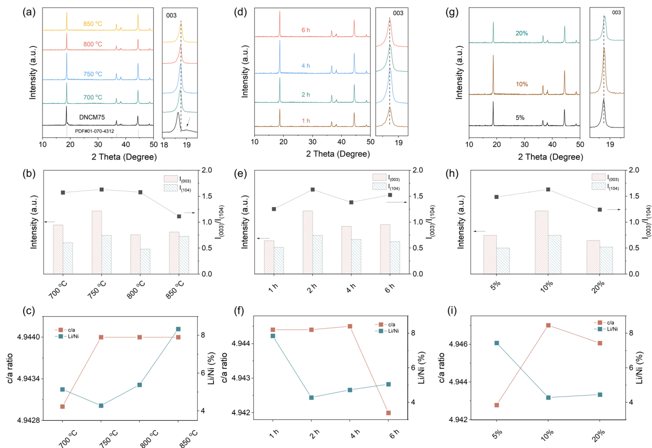
Fig. 2 (a) XRD patterns, (b) I_{(003)}/I_{(104)} ratios and (c) c/a ratios and Li/Ni mixing of RNCM70 sintered at 700 °C, 750 °C, 800 °C, and 850 °C; (d) XRD patterns, (e) I_{(003)}/I_{(104)} ratios and (f) c/a ratios and Li/Ni mixing of RNCM70 sintered at 750 °C for 1, 2, 4, and 6 hours; (g) XRD patterns, (h) I_{(003)}/I_{(104)} ratios and (i) c/a ratios and Li/Ni mixing of RNCM70 sintered at 750 °C with 5%, 10%, and 20% excess Li 2 CO 3 .
