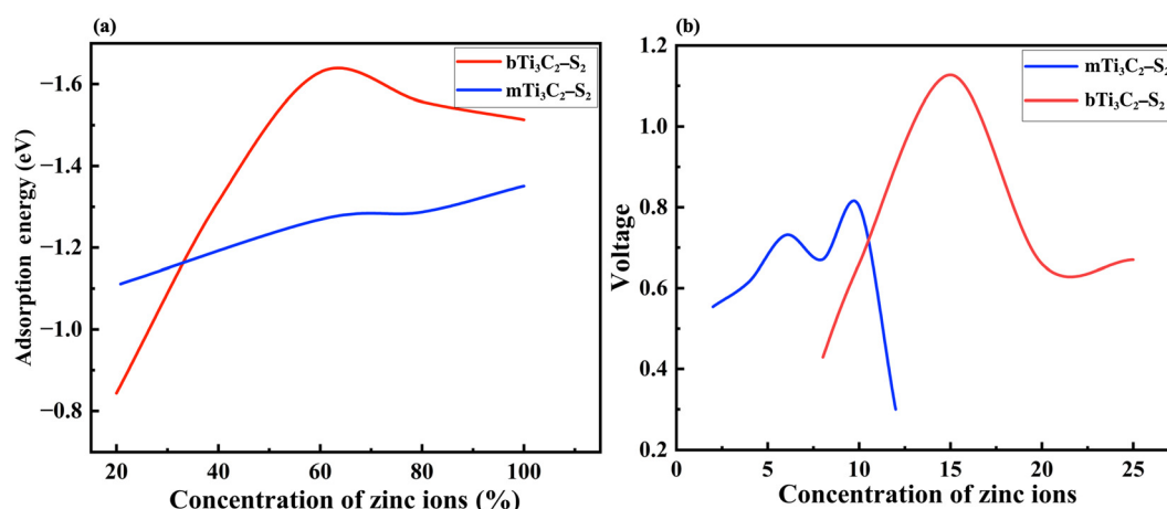
Fig. 3 Representations of (a) the adsorption energy versus Zn-ion concentration curve, showing the variation in adsorption energy with Zn-ion concentration for m \text{Ti}_3\text{C}_2\text{-S}_2 and b \text{Ti}_3\text{C}_2\text{-S}_2 MXene structures and (b) the voltage profile of m \text{Ti}_3\text{C}_2\text{-S}_2 and b \text{Ti}_3\text{C}_2\text{-S}_2 MXene structures with respect to Zn-ion concentration.
