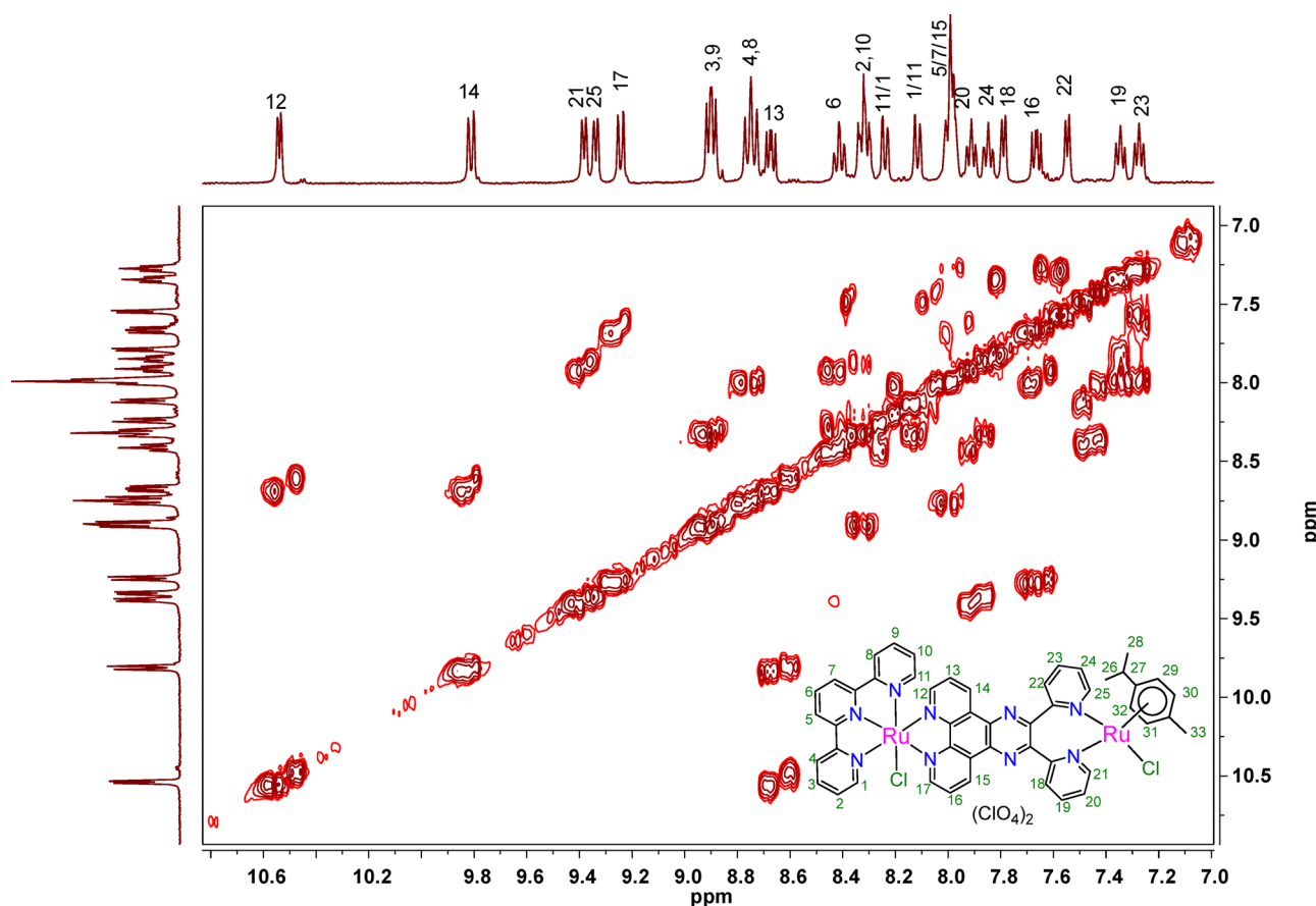
Fig. 3 1 H– 1 H COSY NMR spectrum of the complex 3 in (CD 3 ) 2 SO.
