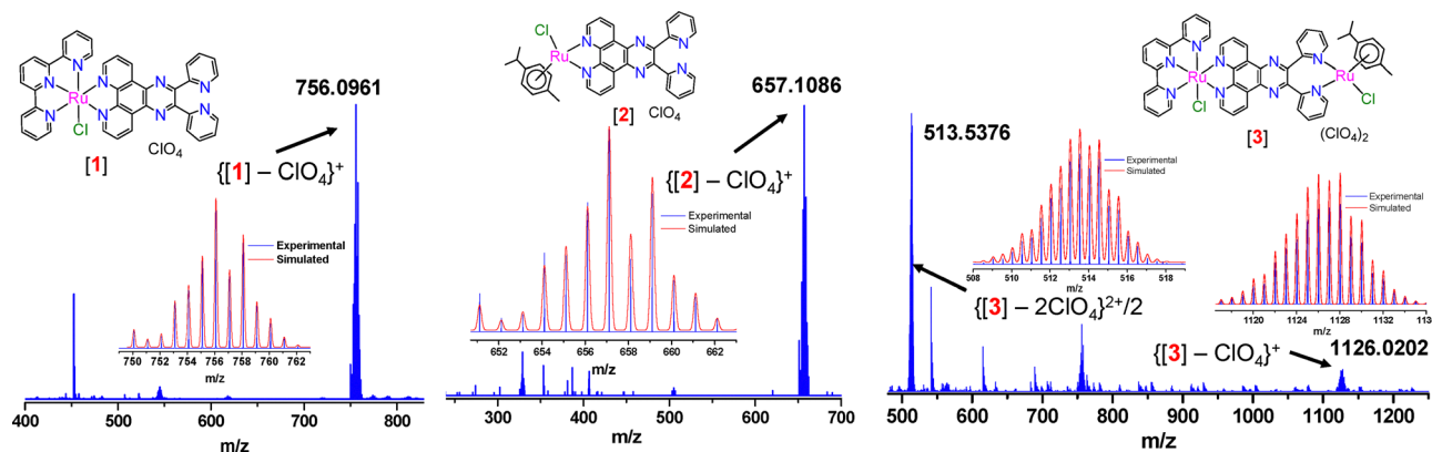
Fig. 2 Molecular structures of the complexes 1–3 and their corresponding HRMS spectra recorded in CH 3 OH. The inset shows the isotopic distribution pattern of the molecular ion peaks.
