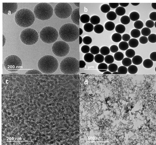
Fig. 1 Electronic microscopy (TEM) images. (a) Porous Stober particles (NPS), (b) nonporous Stober particles, (c) UVM-7, (d) fumed silica.
