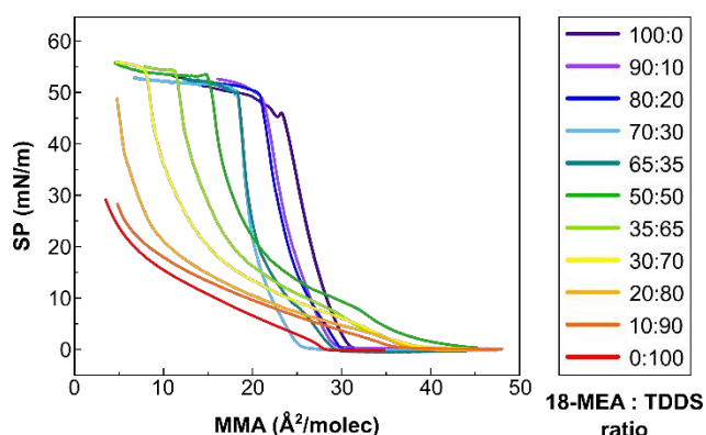
Figure 2. Isotherm trend for different 18-MEA:TDDS molar ratios. Surface pressure is plotted against the mean molecular area, assuming a 2D interface.
