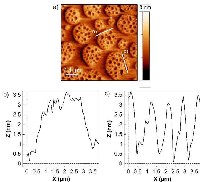
Figure 4. a) AFM height image from deposition of 65:35 mol% 18-MEA:TDDS at SP of 20 mN/m, showing line cuts for b) and c). Scanning size of 12 x 12 μm; b) height profile of the cookie surface and c) height profile of four empty-holes.
