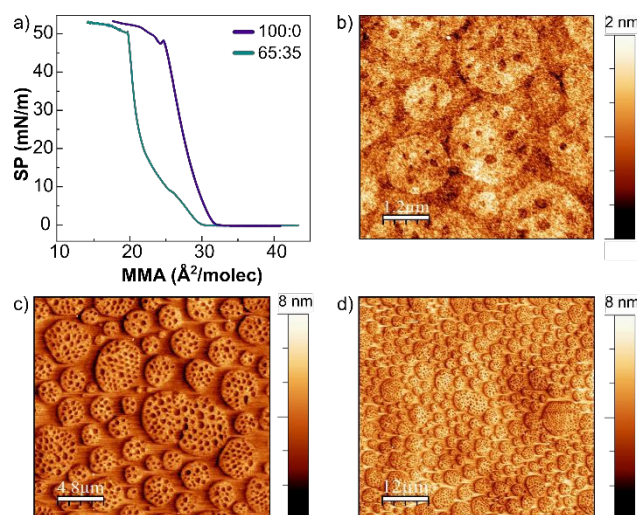
Figure 3. a) Isotherm profile of the 65:35 mol% sample; b), c) and d) AFM height images of 65:35 mol% at a surface pressure of 5 mN/m. Scanning size of 6 x 6 μm, 24 x 24 μm and 60 x 60 μm, respectively.
