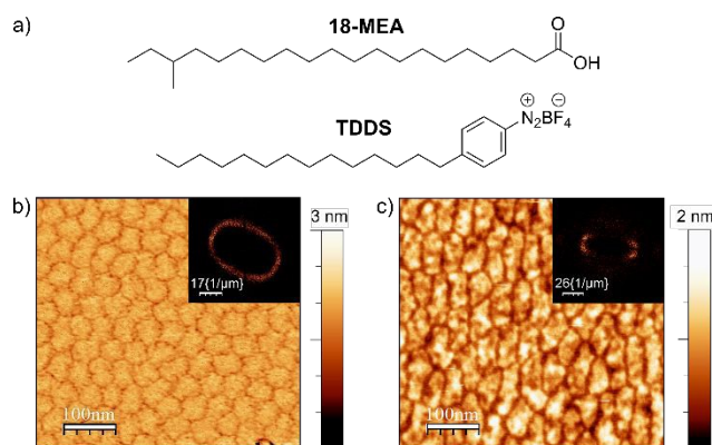
Figure 1. a) Molecular structures of the organic compounds: 18-methyleicosanoic acid (18-MEA, top) and the diazonium salt TDDS (bottom); b) AFM height image of monodisperse nanodomains of pure 18-MEA deposited at 20 mN/m; c) AFM height image of a mixed monolayer of 18-MEA:TDDS (90:10 mol%) deposited at 20 mN/m. Scan area: 500 × 500 nm. Insets in the top right corners show the corresponding Fourier transforms.
