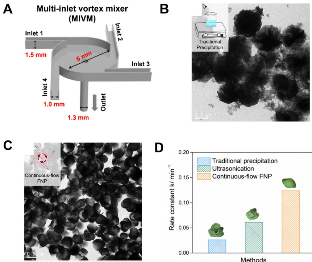
Fig. 11 (A) Diagram of the four-stream MIVM. Morphological comparison of \text{BiOCl}_{0.75}\text{Br}_{0.25} samples processed by (B) traditional nanoprecipitation, (C) FNP. (D) Comparison of kinetic rate constants of the \text{BiOCl}_{0.75}\text{Br}_{0.25} photocatalysts processed by different methods for TC degradation. Adapted with permission from ref. 160. Copyright 2024 Elsevier. 160
