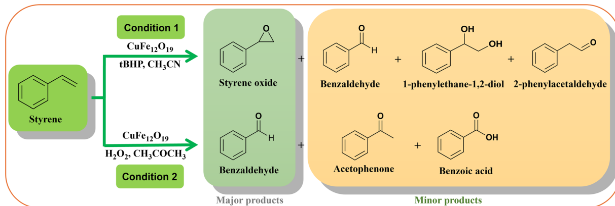
Scheme 2 Catalytic oxidation of styrene in the presence of t BHP or \text{H}_2\text{O}_2 .
