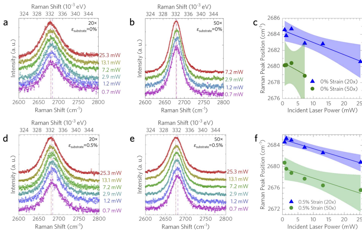
Fig. 6 Power dependent Raman spectra for graphene on copper (method 2). Incident laser power dependent ( P = 0.7 – 25.3 mW) Raman spectra taken using (a) 20 \times and (b) 50 \times objectives. (c) 2D peak position for 0% substrate engineering strain using 20 \times (blue triangles) and 50 \times (green circles) objectives. (d and e) Power dependent Raman spectra and (f) peak positions at 0.5% substrate engineering strain. Linear fits to the data are shown along with the 99% confidence interval bands.
