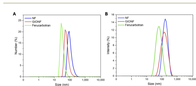
Fig. 1 Hydrodynamic diameter of NF, GIONF, and ferucarbotran as measured by (A) intensity and (B) number-based distribution DLS.
