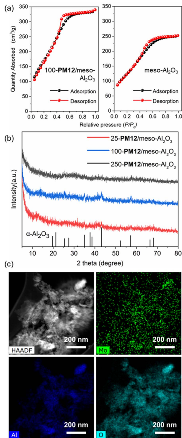
Fig. 2 (a) N 2 adsorption-desorption isotherms (77 K) of 100- PM12 / \text{meso-Al}_2\text{O}_3 and \text{meso-Al}_2\text{O}_3 ; (b) XRD spectra of varying loading amounts of POMs as x\text{-PM12/meso-Al}_2\text{O}_3 ; (c) STEM EDS-mapping images of 100- PM12 / \text{meso-Al}_2\text{O}_3 .
