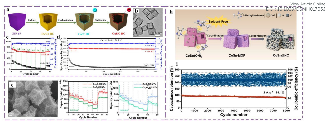
Figure 6. The applications of MOF derivatives for LIB, SIBs, and PIBs. (a) Synthetic process, (b) TEM image, (c) rate and (d) cycle performance of CoS/C HC. [49] Copyright © 2023, Elsevier. (e) SEM image of Co@CNTs; the rate performances of Co 3 O 4 @CNTs and CoS 2 @CNTs for (f) LIB and (g) SIB. [75] Copyright © 2024, American Chemical Society. (h) Schematic illustration for synthetic carbon-coated CoSn alloy (CoSn@NC) and (i) the cycle performance of Li-ion capacitors. [76] Copyright © 2024, Elsevier.
