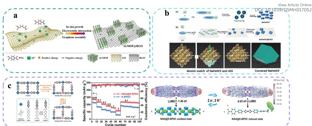
Figure 5. The applications of MOF composites for LIB, SIBs, and PIBs. (a) Schematic illustration of the preparation processes of Al-MOF@RGO composites and the electronic conductivity and transport ability of Li + ions. [65] Copyright © 2023, Elsevier. (b) Structural diagrams of cubic and cornered NaFeHCF and TEM images. [70] Copyright © 2024, Wiley–VCH. (c) Schematic illustration to prepare NiSA@K-BPDC and the chemical structure, ESP images, and LUMO energy levels of NiSA@K-BPDC anodes during cycling. [71] Copyright © 2024, Wiley–VCH.
