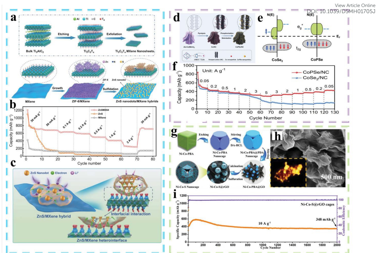
Figure 7. The applications of MOF derivative composites for LIB, SIBs, and PIBs. (a) Schematic illustration for the synthesis of ZnS/MXene hybrids; (b) rate performance and (c) Interfacial interaction mechanism. [97] Copyright 2021 Springer Nature. (d) The synthesis process of the CoPSe/NC composite; (e) Energy level diagrams of the frontier molecular orbitals for pyrite-phase \text{CoSe}_2 and \text{CoPSe} structures; (f) Rate performance. [102] Copyright © 2021, Wiley–VCH. (g) Schematic illustration of the Ni-Co-S@rGO cage nanocomposites; (h) TEM image; (i) cycle performance. [103] Copyright © 2022, Wiley–VCH.
