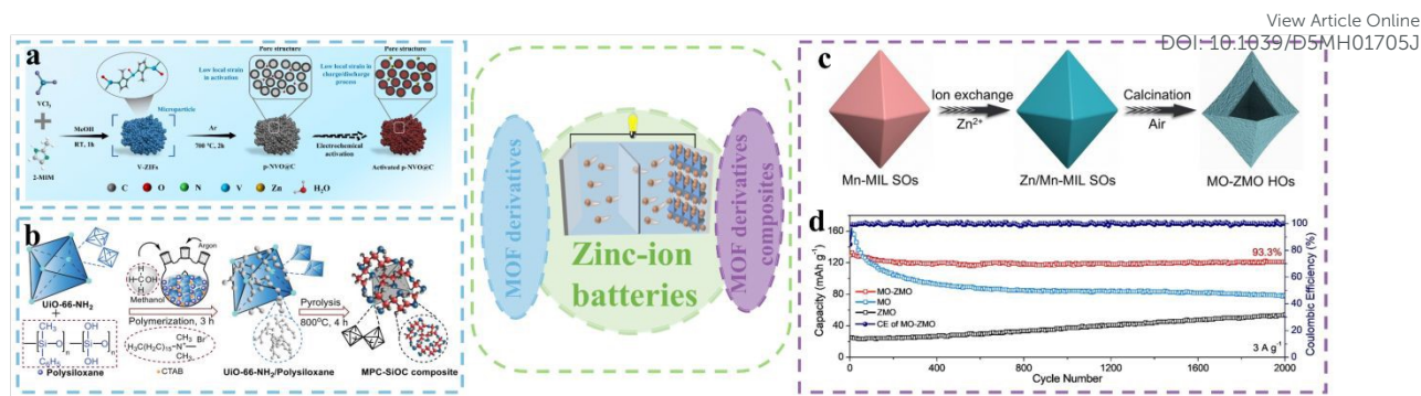
Figure 11. MOF-based materials for ZIBs. (a) Synthesis and structure of p-NVO@C. [171] Copyright © 2024, Elsevier. (b) Schematic presentations of the synthesis of MPC-SiOC. [173] Copyright © 2024, Wiley–VCH. (c) Schematic illustration of the synthetic process of MO–ZMO HOs; (d) the long cycle performance of at current density of 3 A g -1 . [174] Copyright © 2021, Wiley–VCH.
