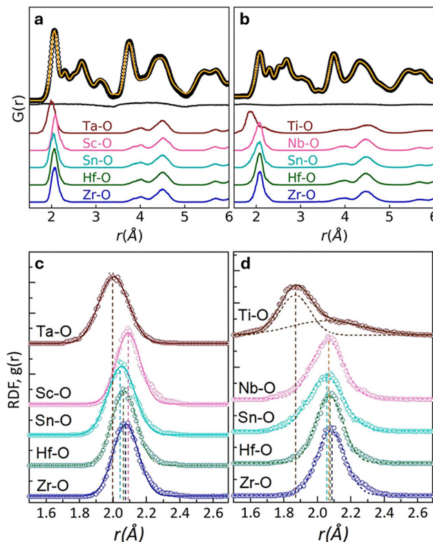
Fig. 7 Experimental G(r) (black circles) and Reverse Monte Carlo simulation (orange lines) for (a) Nd 2 M 2 O 7 with M = Ta, Sc, Sn, Hf, Zr, and (b) Nd 2 M 2 O 7 with M = Ti, Nb, Sn, Hf, Zr, with partial pair correlation functions from models shown below as separate, labeled, colored lines. Gaussian peak fitting of the first M–O pair–pair correlation peaks from the RMC partial PDF distributions in (c) Nd 2 M 2 O 7 with M = Ta, Sc, Sn, Hf, Zr, and (d) Nd 2 M 2 O 7 with M = Ti, Nb, Sn, Hf, Zr. A double deconvoluted Gaussian peak was used to fit the Ti–O bond distribution peaks. Reprinted with permission from Jiang et al. J. Am. Chem. Soc. 2021, 143 , 11, 4193–4204. Copyright 2021, ACS.
