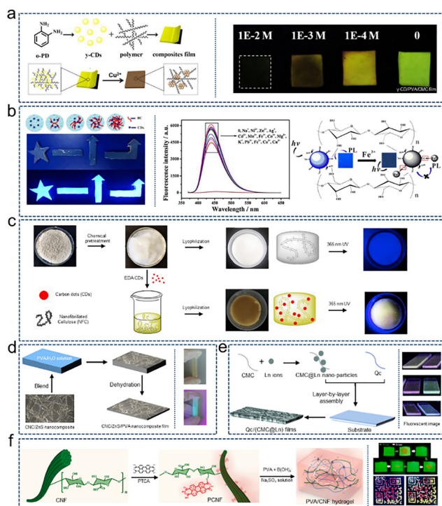
Fig. 4 Design strategy and phenomena for achieving extrinsic fluorescence of cellulose. (a) Preparation process of y-CD/PVA/CMC film and fluorescence image of the film interacting with Cu 2+ . [Reproduced with permission from ref. 24. Copyright 2013 The Royal Society of Chemistry.] (b) Fluorescence imaging of bacterial cellulose loaded carbon dot composite materials and the mechanism of specific recognition of Fe 3+ . [Reproduced with permission from ref. 25. Copyright 2017 Elsevier Ltd.] (c) Fabricating process and fluorescent properties of nanofibrillated cellulose and NFC loaded CD composite. [Reproduced with permission from ref. 26. Copyright 2020 Elsevier B.V.] (d) Preparation process of CNC/ZnS/PVA nanocomposite film and the fluorescence spectra. [Reproduced with permission from ref. 27. Copyright 2019 Springer Nature B.V.] (e) Preparation process of Qc/(CMC@Ln) films and fluorescence imaging. [Reproduced with permission from ref. 28. Copyright 2017 Elsevier Ltd.] (f) Production process of the PVA/CNF hydrogel and the fluorescent image of anti-counterfeiting. [Reproduced with permission from ref. 29. Copyright 2024 Elsevier B.V.]
