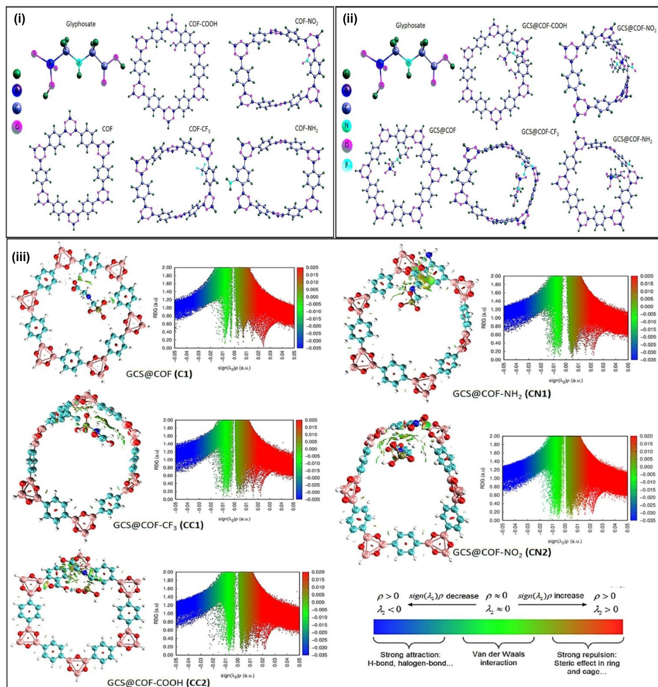
Figure 12: (i) Optimized structures of the GCS with the pure and functionalized COFs, (ii) Optimized structures of stable configurations of the stable complexes (complexes of the COFs with GCS) studied at M06-2X/ LanL2DZ level of theory, and (iii) 3D NCI isosurface and the 2D RDG scatter maps for all studied complexes. Reproduced from ref. 233 with permission from Elsevier, Copyright 2025.
