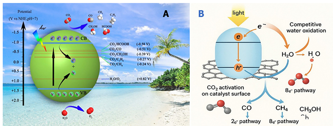
Fig. 2 (A) Band edge alignment and redox potentials for the photocatalytic CO 2 reduction with H 2 O. (B) General mechanism of the graphene-based photocatalytic CO 2 reduction pathways. Reprinted from ref. 22, copyright@2020, RSC.
