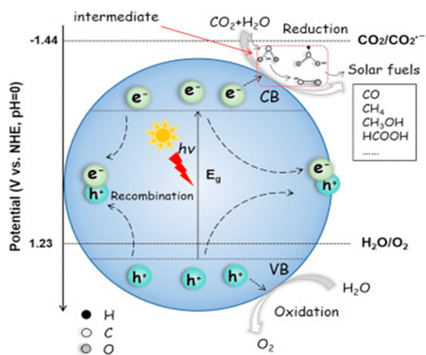
Fig. 3 Schematic of the thermodynamics and kinetics of CO 2 photoreduction. Reprinted from ref. 26, copyright@2020, Elsevier.
