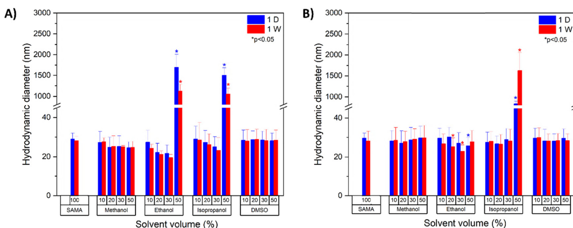
Fig. 1 Hydrodynamic diameters. Obtained by DLS, diameters of BMV and CCMV after being incubated in the solvent mixtures for 1 day (blue) and 7 days (red). (A) Hydrodynamic diameters of BMV with solvent mixtures and SAMA buffer. (B) Hydrodynamic diameters of CCMV with solvent mixtures and SAMA buffer. Bars represent the average diameter, and error bars represent the standard deviation (SD). Means and standard deviations are reported in Table S1. Statistical analyses One-way ANOVA, Tukey test, * P < 0.05.
