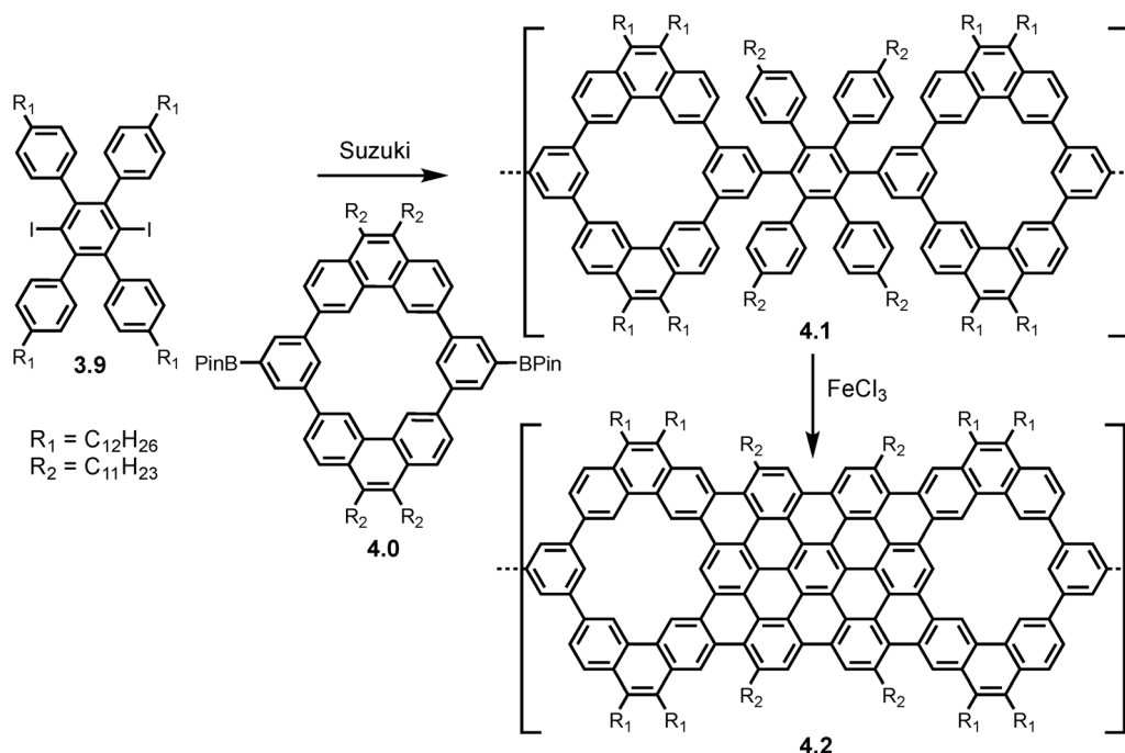
Scheme 6 Synthesis of pGNR 4.2 from \text{A}_2\text{B}_2 Suzuki polymerisation of 3.9 and 4.0 . Reproduced from ref. 46 with permission from [Wiley], copyright [2023].
