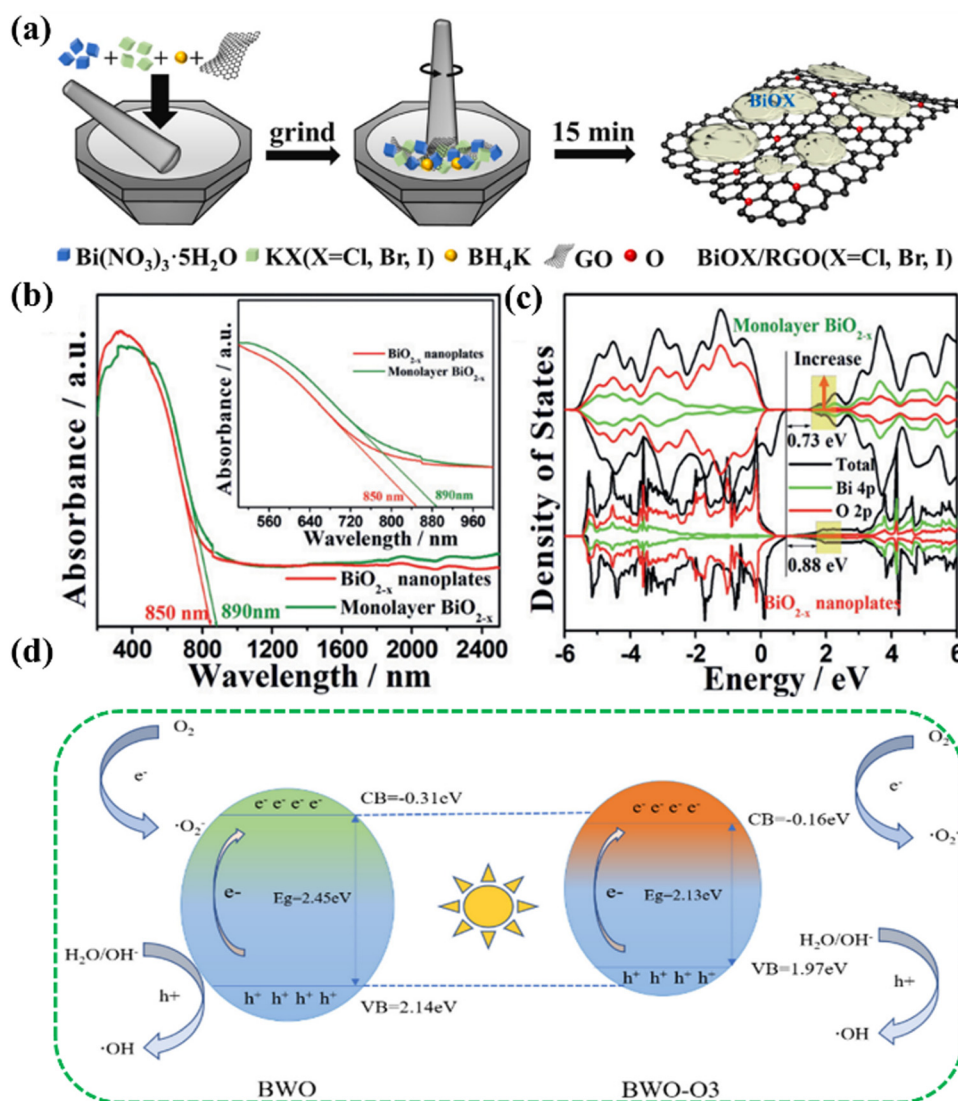
Fig. 3 (a) Synthesis of the BiOX/RGO ( \text{X} = \text{Cl}, \text{Br} and \text{I} ) composite. 6 Copyright 2021, Elsevier. (b) UV/vis-NIR DRS of \text{BiO}_{2-x} . (c) Total density of states (TDOS) of \text{BiO}_{2-x} . 68 Copyright 2017, Wiley. (d) Schematic of \text{Bi}_2\text{WO}_6 with/without oxygen vacancies. 69 Copyright 2023, Elsevier.
