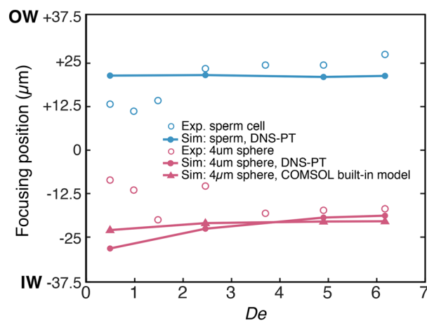
Fig. 2 Lateral focusing position of particles in a spiral channel. Experimental results for sperm cell and 4 \mu\text{m} spheres are compared against the DNS-PT modelling results, and the COMSOL built-in inertial lift force model.
