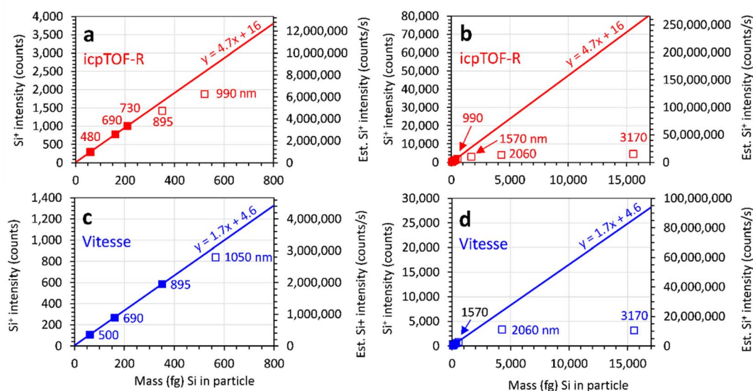
Fig. 3 ^{28}\text{Si}^+ signal in counts (left y-axis) and estimated counts per s (right y-axis) produced by engineered \text{SiO}_2 particle suspensions measured by: (a and b) TOFWERK iCP-TOF-R and (c and d) Nu Instruments Vitesse spICP-TOFMS using optimized sensitivity for particles with: (a and c) masses less than 800 fg and (b and d) masses less than 17 000 fg. The nominal particle diameter is shown next to each point. Filled symbols indicate particles used to calculate the linear regression line while open symbols indicate particles not used to calculate the linear regression line.
