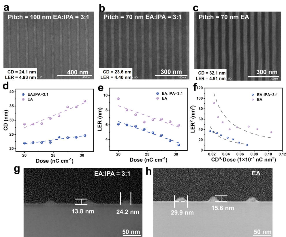
Fig. 2 SEM images of the Sn4-MB 's (a) 100 nm and (b) 70 nm pitch lines when developed with EA:IPA = 3 : 1 at 26 \text{ nC cm}^{-1} exposure doses; (c) SEM image of the Sn4-MB 's 70 nm pitch lines when developed with EA at 26 \text{ nC cm}^{-1} exposure dose; relation of 100 nm pitch line (d) CD and (e) LER with dose after EA:IPA = 3 : 1 and EA development of Sn4-MB films upon EBL line-exposure; (f) Z constant of Sn4-MB 's 100 nm pitch lines under EA:IPA = 3 : 1 and EA development; profile of Sn4-MB 's lines when developed with (g) EA:IPA = 3 : 1 and (h) EA.
