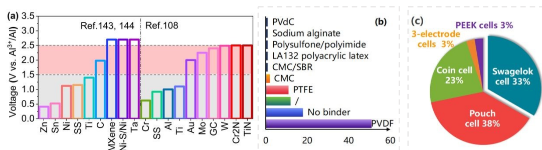
Figure 16. a) The oxidative stability, in terms of the voltage versus \text{Al}/\text{Al}^{3+} , of Ni-S/ \text{Ni}^{143} , MXene and other various current collector materials 144 in \text{AlCl}_3/[\text{EMIm}]\text{Cl} electrolyte with molar ratios of 1.3 (left) and 2.0 (right). Adapted from Wang, S. et al., Adv Sci (Weinh) 108 . Licensed under CC BY 4.0. ©2018 Wiley. b) Number of publications reporting various binders used in AGDIBs based on literature survey ('/' indicates not mentioned). c) Cell configurations applied in AGDIBs from the literature survey.
