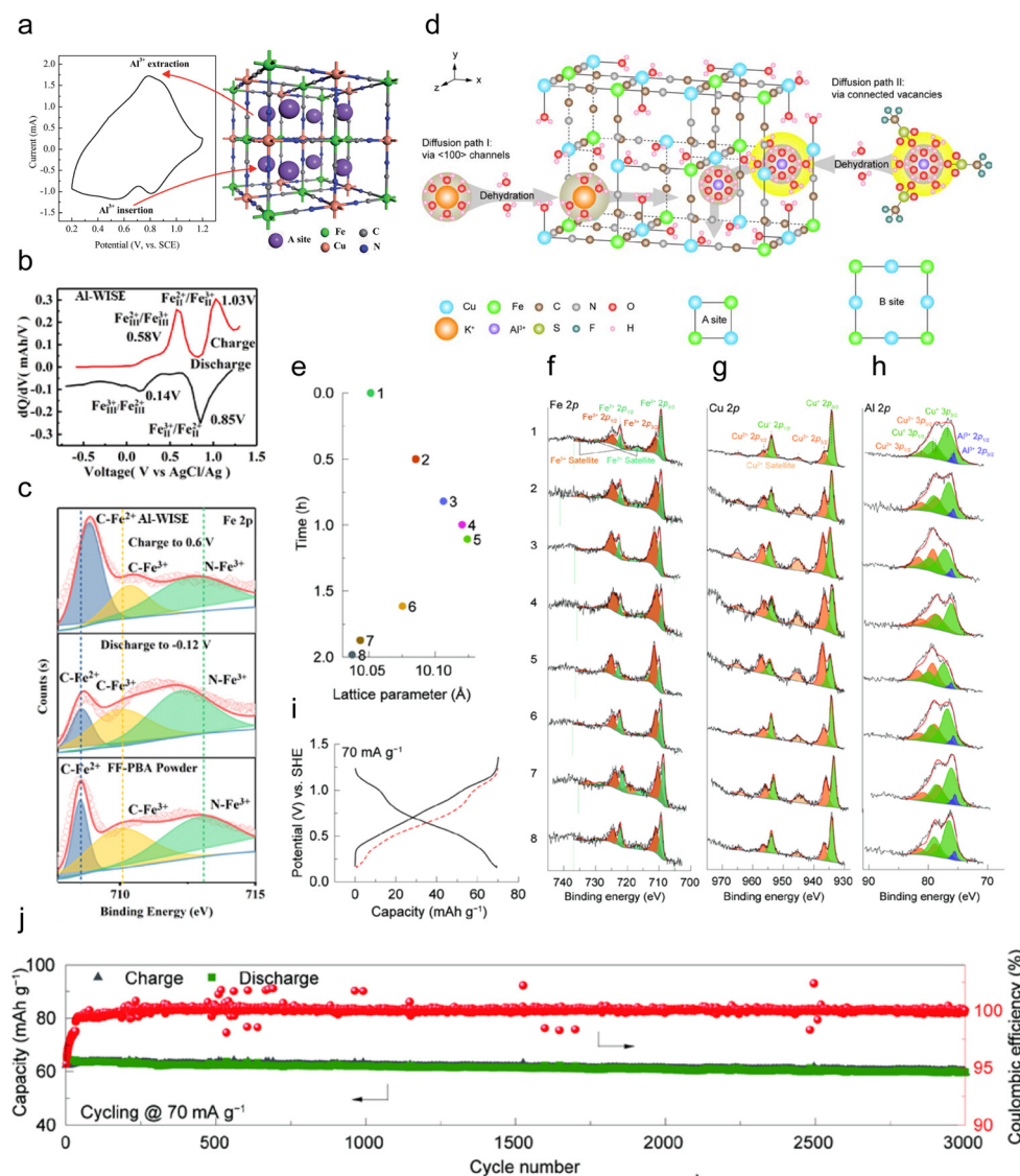
Fig. 5 (a) CV curve and structure of the CuHCF nanoparticle. 102 Copyright 2015, The Royal Society of Chemistry. (b) The differential profiles at the 50 th cycle, and (c) XPS spectrum of the \text{FeFe}(\text{CN})_6 electrode in different charge–discharge states (pristine, discharge to -0.12 V and charge to 0.6 V) in the 5\text{ M Al}(\text{CF}_3\text{SO}_3)_3 water-in-salt electrolyte. 105 Copyright 2019, American Chemical Society. (d) Crystal structure of the CuHCF with two possible diffusion paths. Diffusion path I was through \langle 100 \rangle channels, and path II was through enlarged open channels by the connected ferro- and ferricyanide vacancies. (e–h) XPS patterns of the Fe 2p (f), Cu 2p (g), and Al 2p (h) for the electrodes. (i) GCPL curve at a current rate of 70\text{ mA g}^{-1} . The red dash line was the flipped discharge curve. (j) Long-term stability at 70\text{ mA g}^{-1} . 106 Copyright 2023, Elsevier B.V.
