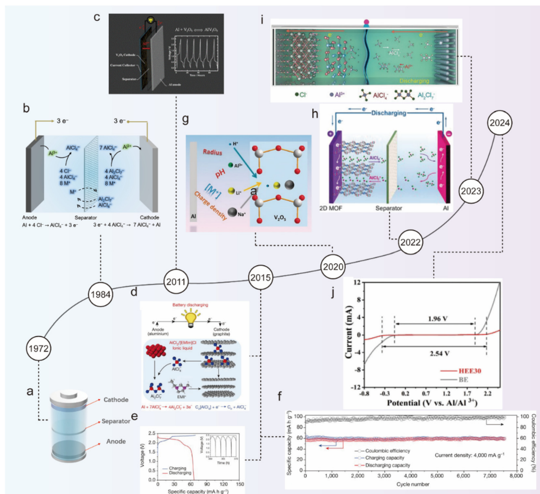
Fig. 2 A brief history of AlIBs. Schematic illustration of (a) an Al||C|| 2 secondary battery with the NaCl/KCl/AlCl 3 molten electrolyte, (b) an Al||Al battery with the AlCl 3 /MEtCl ionic liquid electrolyte, and (c) an Al||V 2 O 5 battery with the AlCl 3 /EMImCl ionic liquid electrolyte. 40 Copyright 2011, The Royal Society of Chemistry. (d) Schematic illustration, (e) galvanostatic charge and discharge curves, and (f) long-term stability test of an Al||graphite battery with the AlCl 3 /EMImCl ionic liquid electrolyte. 45 Copyright 2015, Springer Nature. (g) Schematic illustration of a reversibly co-inserted Al 3+ /H + in an Al||V 2 O 5 battery with the 2 M Al(OTf) 3 aqueous electrolyte. 46 Copyright 2020, Wiley-VCH. (h) Schematic illustration of an Al||MOF battery with the AlCl 3 /EMImCl ionic liquid electrolyte. 47 Copyright 2022, Wiley-VCH. (i) Schematic illustration of an Al||CoSe 2 /MXene battery with the AlCl 3 /EMImCl ionic liquid electrolyte. 48 Copyright 2023, Wiley-VCH. (j) LSV curves of the BE and HEE30 electrolytes at a scan rate of 10 mV s -1 . 49 Copyright 2024, Wiley-VCH.
