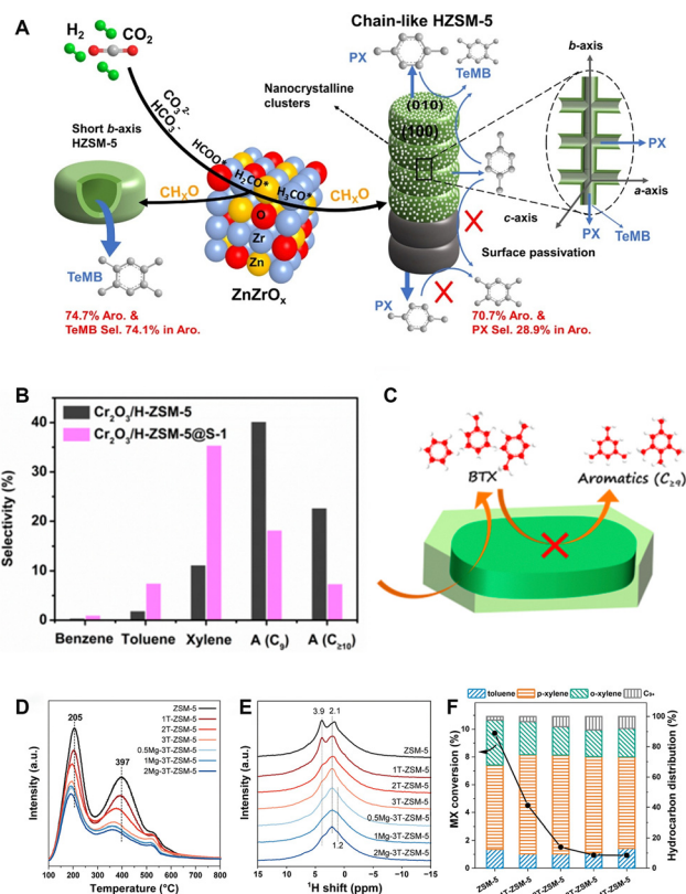
Fig. 10 (A) Utilization of ZSM-5 with chain-like and hollow morphology in the CO 2 -to-aromatics reaction. Reprinted with permission from Wang et al. Copyright (2021), Elsevier B.V. 53 (B) and (C) Catalytic performance of the core-shell structured ZSM-5@S-1 in the CO 2 -to-aromatics reaction. Reprinted with permission from Wang et al. Copyright (2019), American Chemical Society. 55 (D) NH 3 -TPD profiles, (E) 1 H NMR spectra and (F) isomerization of meta-xylene of ZSM-5 co-modified with MgO and an inert shell. Reprinted with permission from Qu et al. Copyright (2023), The Royal Society of Chemistry. 61
