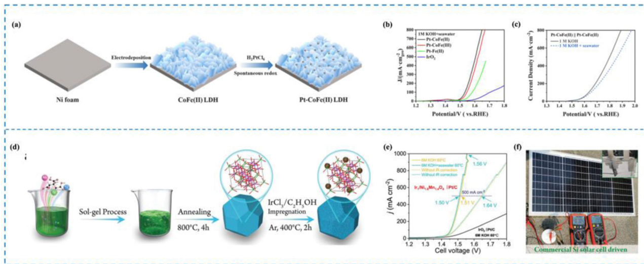
Fig. 11 Synthesis and selectivity of Pt–CoFe(II) LDHs (a)–(c) and Ir 1 /Ni 1.6 Mn 1.4 O 4 (d)–(f). (a) Synthesis of Pt–CoFe(II) LDHs. (b) AEMWE curve in seawater for Pt–CoFe(II) LDHs. (c) Overall water/seawater splitting performance of Pt–CoFe(II) LDHs in different electrolytes. (d) Synthesis of Ir 1 /Ni 1.6 Mn 1.4 O 4 . (e) AEMWE curve in seawater for Ir 1 /Ni 1.6 Mn 1.4 O 4 . (f) Optical image of Ir 1 /Ni 1.6 Mn 1.4 O 4 ||Pt/C electrode pairs driven by silicon PV in 0.5 M KOH + seawater. 195,196 This figure has been adapted/reproduced from ref. 195 and 196 with permission from Elsevier and John Wiley and Sons, copyright©2022 Elsevier B.V. All rights reserved. Copyright©2022 The Authors. Advanced Science published by Wiley-VCH GmbH.
