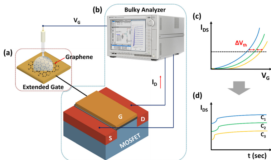
Fig. 1 Conventional setup for operating a remote-gate graphene sensor. (a) A remote gate separated from a MOSFET transducer. (b) A transducer and an analyzer for acquiring sensor signals. (c) Transfer characteristic curves observed in typical operation. (d) Real-time monitoring of I_{\text{DS}} for portable sensor operation.
