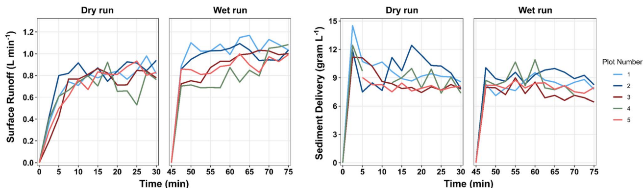
Fig. 3 Surface runoff and sediment flux during the rainfall simulations across the five plots ( n = 5 ). Time 0 indicates the commencement of surface runoff. Missing data points in plot 4 are visible, these values were outliers and were excluded from the analysis.
