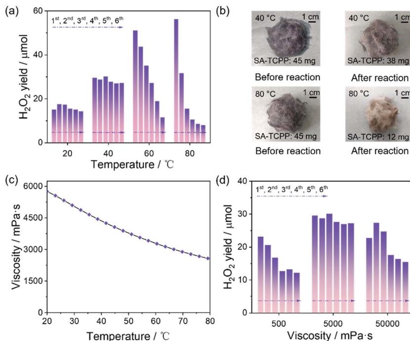
Fig. 5 (a) \text{H}_2\text{O}_2 yields and cycling stability of PDMS/SA-TCPP/QW composites at various reaction temperatures (PDMS viscosity: 5000 mPa s). (b) Corresponding macroscopic photographs of PDMS/SA-TCPP/QW composite before and after reactions at 40 °C and 80 °C, illustrating the morphological changes under thermal conditions. (c) Temperature-dependent viscosity profile of PDMS (5000 mPa s) under atmospheric pressure. (d) \text{H}_2\text{O}_2 yields and cycling stability of PDMS/SA-TCPP/QW composite at various PDMS viscosities. Reaction temperature: 40 °C. Solution: 30 mL \text{H}_2\text{O} , pH = 7, SA-TCPP catalyst loading: 45 mg, \text{O}_2 bubbling, reaction time: 4 h, light source: Xe lamp with a 420 nm cut-off filter.
