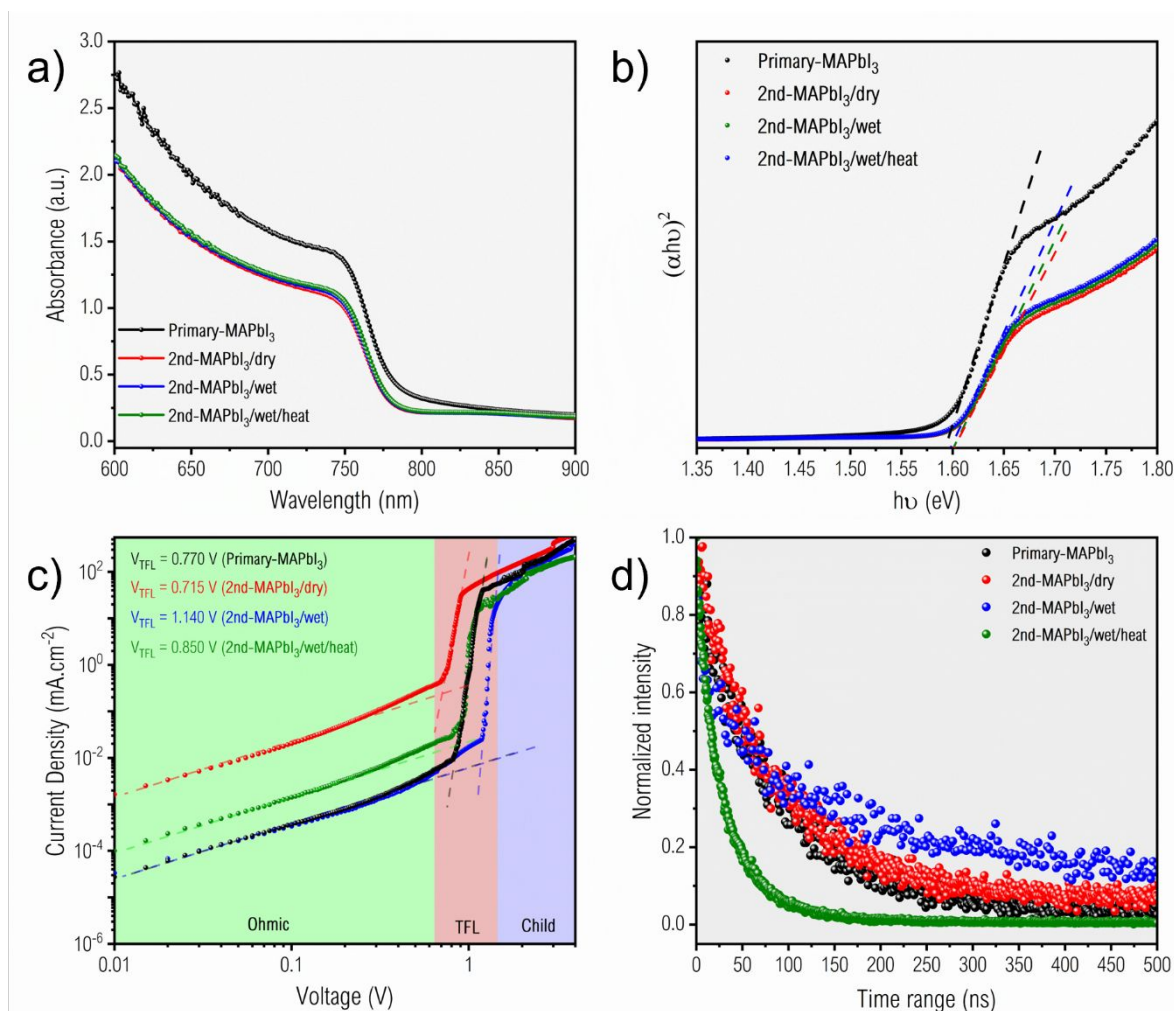
Figure 8: a) UV-vis absorption spectra, b) Tauc-plot, c) the SCLC curves and d) the TRPL spectra of Glass/Al 2 O 3 /PVSK film of Primary-MAPbI 3 , 2nd-MAPbI 3 /dry , 2nd-MAPbI 3 /wet and 2nd-MAPbI 3 /wet/heat films
