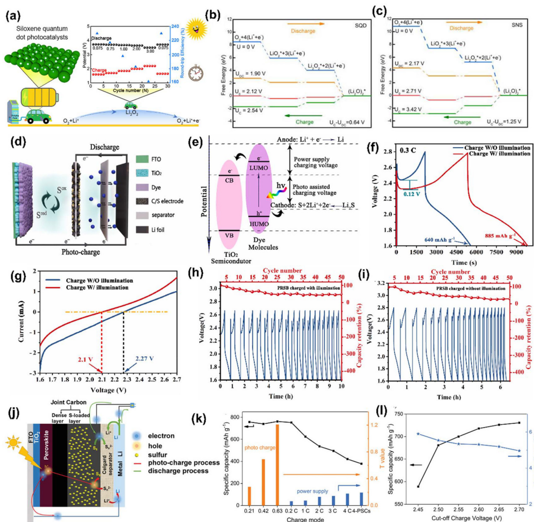
Fig. 10 (a) Schematic representation of Li–O 2 PARB with a siloxene quantum dot (b–c) energy diagrams for the discharge–charge reactions on the active surface of SQD and SNSs. 46 Copyright: 2023 American Chemical Society. (d) Device structure, (e) energy diagram, (f) GCD curves at 0.3C, (g) LSV curves with and without illumination, (h) cycling performance with illumination, and (i) cycling performance without the illumination of the Li–S PARB. 47 Copyright: 2023 Elsevier. (j) Schematic diagram, (k) discharge capacities (black line) and T values (blue and yellow columns) of the battery under different charge modes, (l) discharge capacity and overall efficiency of different cut-off photocharge voltage of the fabricated PSC–Li–S battery. 48 Copyright: 2019 Wiley.
