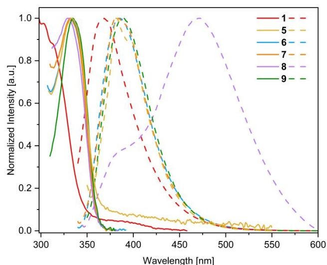
Figure 4. Normalized absorption- (compact) and emission (dashed) spectra of 1 and 5–9 .
