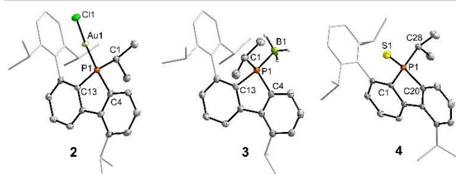
Figure 1. Molecular structures of 2 (left), 3 (middle) and 4 (right). Ellipsoids drawn at 50 % with C-H atoms omitted, Dipp- and one of the i Pr-groups rendered as wire-frame for clarity. Selected bond lengths [Å] and angles [°] of 2 : C1-P1 1.845(2), C4-P1 1.798(2), C13-P1 1.805(2), P1-Au1 2.2247(6), Cl1-Au1 2.2885(6); C4-P1-C13 91.83(10), C4-P1-C1 106.46(10), C13-P1-C1 105.84(10), C4-P1-Au1 114.61(7), C13-P1-Au1 121.62(7), C1-P1-Au1 113.71(8); C5-C4-P1-C13 179.9(2). 3 : P1-C4 1.7991(13), P1-C13 1.8102(13), P1-C1 1.8435(14), P1-B1 1.9269(16); C4-P1-C13 91.52(6), C4-P1-C1 108.29(6), C13-P1-C1 107.20(6), C4-P1-B1 111.38(7), C13-P1-B1 121.08(6), C1-P1-B1 114.62(7); C13-P1-C4-C9 -178.84(12) ; 4 : P1-C1 1.809(1), P1-C20 1.797(1), P1-C28
