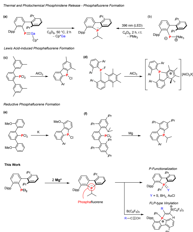
Scheme 1. (a) Thermal phosphinidene release from a phosphagallene, (b) Photochemical PMe 3 release from Dipp TerP(PMe 3 ); (c,d) Lewis acid induced phosphafluorene formation in terphenyl-substituted halophosphanes; (e,f) Reductive approaches towards phosphafluorenes from dichlorophosphanes (e, f); and summary of this work.
