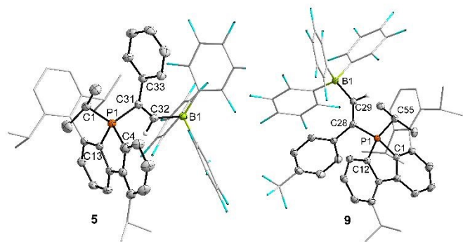
Figure 2. Molecular structures of 5 and 9 . Ellipsoids drawn at 50 % with C-H-atoms omitted (except those at C32 ( 5 ) and C29( 9 )), Dipp-, C 6 F 5 -, CF 3 - and one of the i Pr-groups rendered as wire-frame for clarity. Selected bond lengths [Å] and angles [°] of 5 : P1–C4 1.7915(18), P1–C13 1.8014(16), P1–C1 1.8282(18), P1–C31 1.8282(17), B1–C32 1.648(2), C31–C32 1.344(2); C4–P1–C13 93.34(8), C4–P1–C1 110.49(8), C13–P1–C1 113.17(8), C4–P1–C31 107.19(8), C13–P1–C31 112.12(7), C1–P1–C31 117.64(8), C32–C31–P1 112.79(12), C31–C32–B1 138.96(15); C4–P1–C31–C32 65.08(14). 9 : C1–P1 1.8007(14), C12–P1 1.7807(14), C28–P1 1.7969(13), C55–P1 1.8326(14), C28–C29 1.3433(19), C29–B1 1.642(2), C12–P1–C28 108.96(6), C12–P1–C1 93.52(6), C28–P1–C1 122.55(6), C12–P1–C55 108.64(7), C28–P1–C55 113.19(6), C1–P1–C55 107.71(6), C29–C28–P1 116.86(10), C28–C29–B1 136.79(13); C29–C28–P1–C12 137.25(11).
