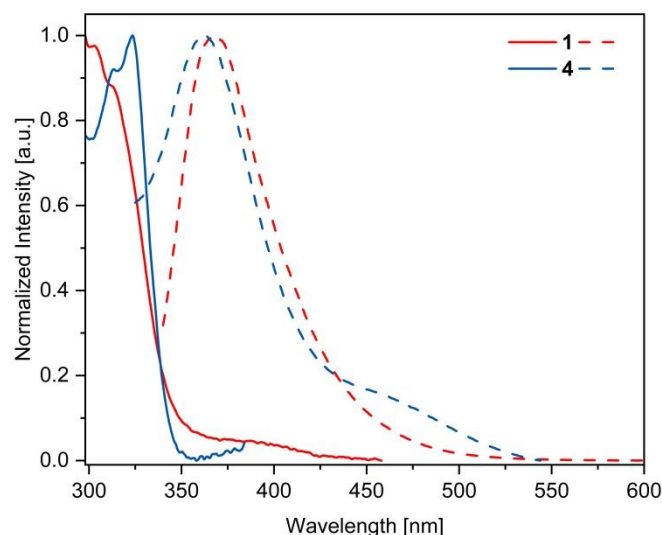
Figure 3. Normalized absorption- (compact) and emission (dashed) spectra of 1 and 4 .
