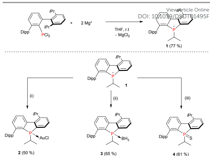
Scheme 2. Synthesis of phosphafluorene 1 (top). Functionalization of the phosphorus center in 1 : (i) \text{AuCl-SMe}_2 , toluene, 16 h, r.t.; (ii) \text{H}_3\text{B-SMe}_2 , n -hexane, 16 h, r.t.; (iii) 1/8 \text{ S}_8 , \text{CH}_2\text{Cl}_2 , 16 h, r.t.
