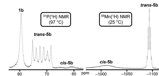
Fig. 8 ^{31}\text{P}\{^1\text{H}\} (left, 202 MHz) and ^{55}\text{Mn}\{^1\text{H}\} (right, 124 MHz) NMR spectra of [(\text{dmpe})_2\text{Mn}(\text{GeHEt}_2)(\text{N}_2)] ( 5b ) at 370 and 298 K, respectively ( d_8 -toluene, \text{N}_2 atmosphere), showing the sextet or quintet arising from the trans isomer due to ^{31}\text{P} – ^{55}\text{Mn} coupling, along with peaks arising from the cis isomer and from (left only) trans - [(\text{dmpe})_2\text{MnH}(\text{=GeEt}_2)] ( 1b ; formed due to reversible \text{N}_2 dissociation from 5b at elevated temperature). The ^{31}\text{P}\{^1\text{H}\} NMR spectrum was obtained at elevated temperature to reduce the extent of quadrupolar collapse for the trans - 5b signal (note that signals for cis - 5b , which are broadened at this temperature, are sharp singlets at low temperature as shown in Fig. S143† due to complete quadrupolar collapse of coupling to ^{55}\text{Mn} and/or slowing of a fluxional process which renders the ^{31}\text{P} atoms equivalent at high temperature).
