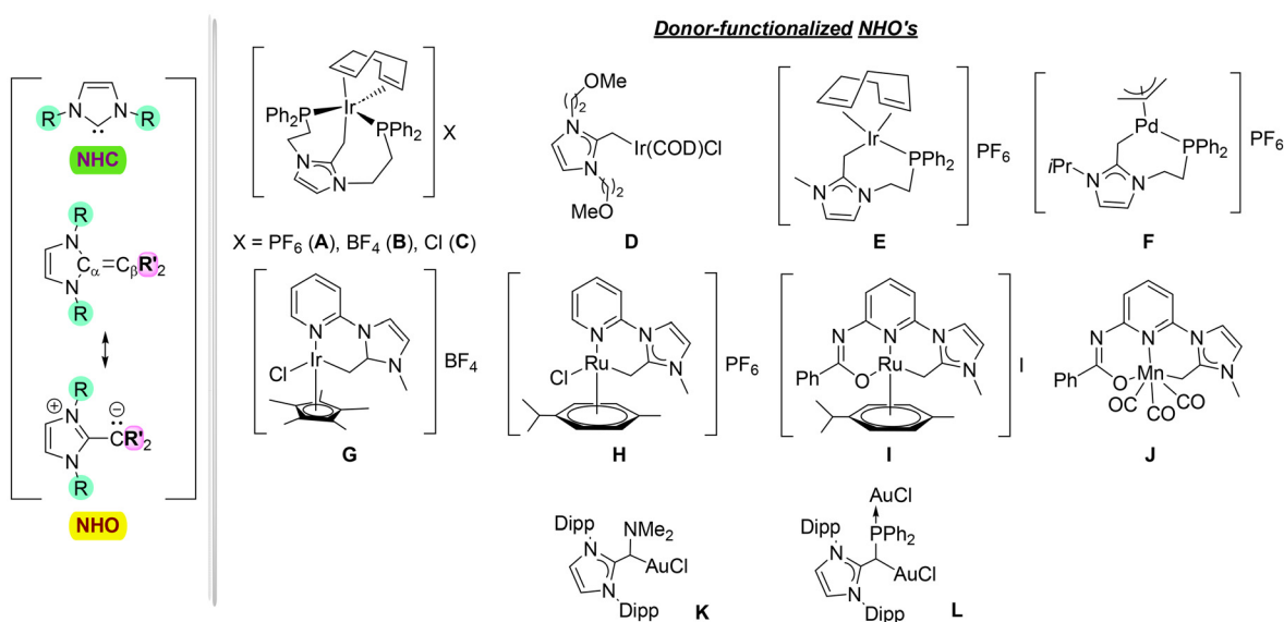
Fig. 1 (left): NHC and NHO frameworks with possible sites for donor functionalization highlighted in green (wingtips) and pink (NHO- C_\beta ). (right): selective examples of donor-functionalized NHO complexes previously known.
